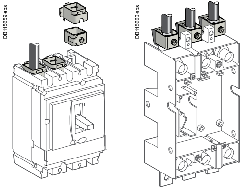
1-cable connector
